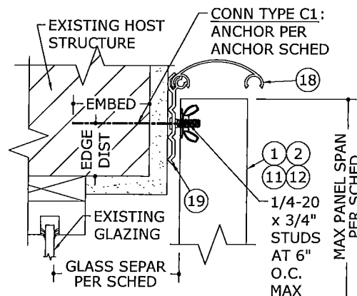
4 MOUNTING SECTION 4 N.T.S. VERT SECTION
