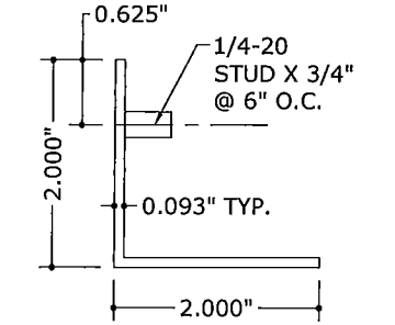
14 ALTERNATE STUD ANGLE 6" = 1'-0"
