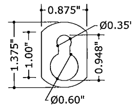
8 KEYHOLE WASHER 6" = 1'-0"
